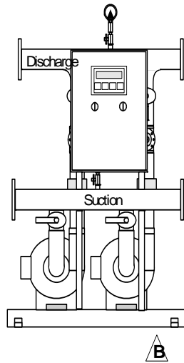
Panel on Pump Side
