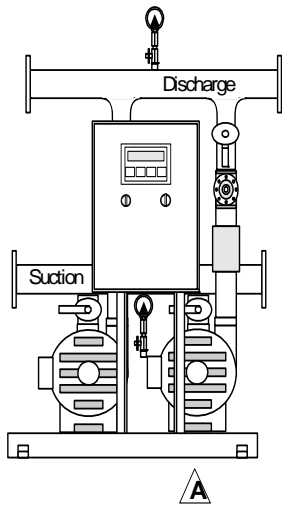
Panel on Motor Side
